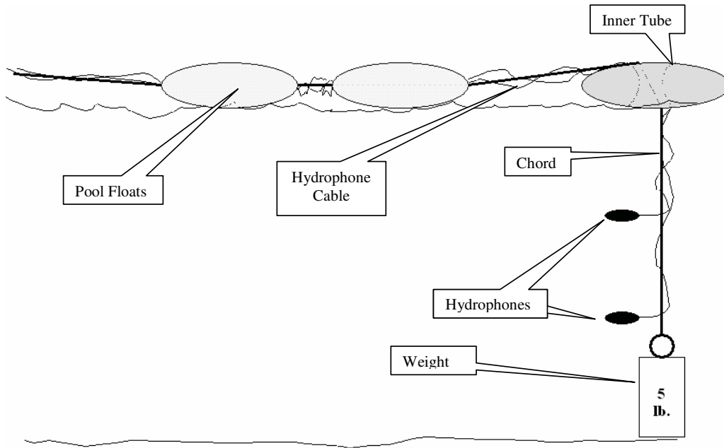
Figure 5: Diagram of hydrophone deployment.
