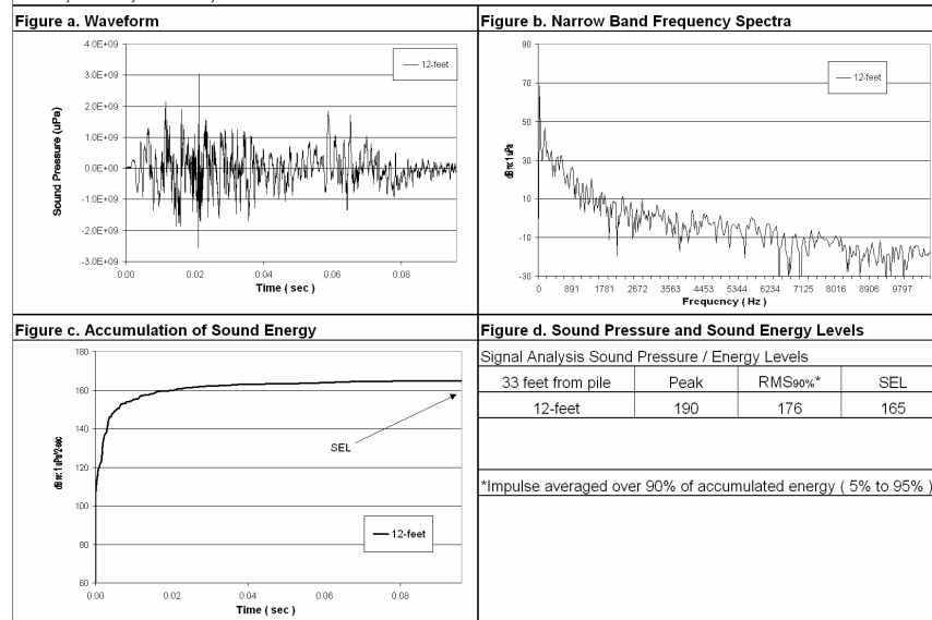
Figure 24: Waveform Analysis of Pile Number 5 Sound Pressure Levels with Wood Pile Cap and Bubble Curtain Off, Midwater and Bottom.
